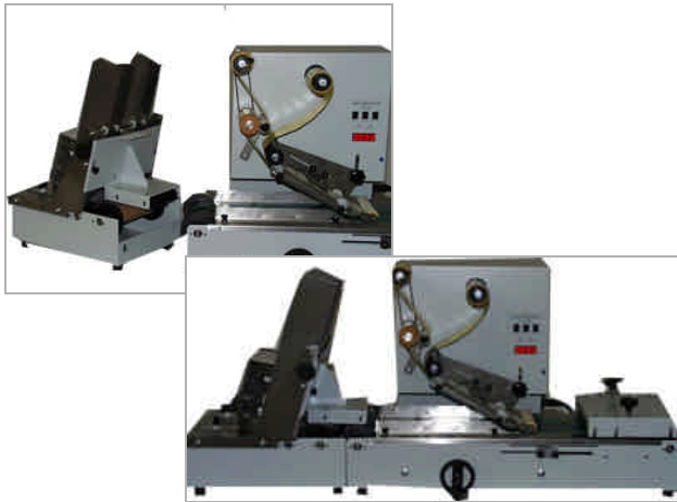
Optional hopper fits easily on the end of the VS350 for dispensing CD jewel cases & sleeves
